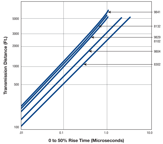
Rise Time
