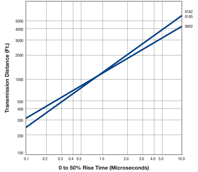
Rise Time
